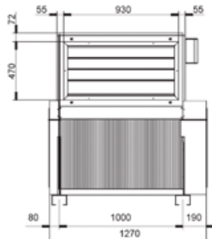
Vista frontal
